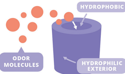
\beta -CYCLODEXTRIN
